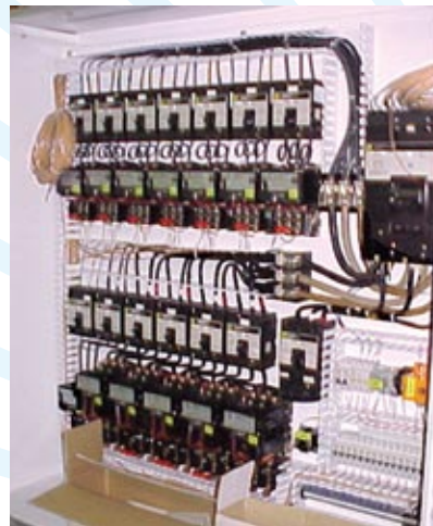
THIS CONTROL PANEL INCLUDED MOTOR STARTERS FOR SEVERAL CONVEYER SYSTEMS IN AN AGRICULTURAL RICE MILL. THE NEMA 12 PANEL INCLUDES AN AC SYSTEM FOR BOTH COOLING AND TO PROTECT THE SYSTEM FROM THE EXTREME DUST ENVIRONMENT.
